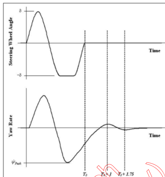
Diagram 1: Steering wheel position and yaw velocity information used to assess lateral stability
